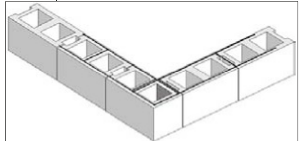
PREFABRICATED CORNER
